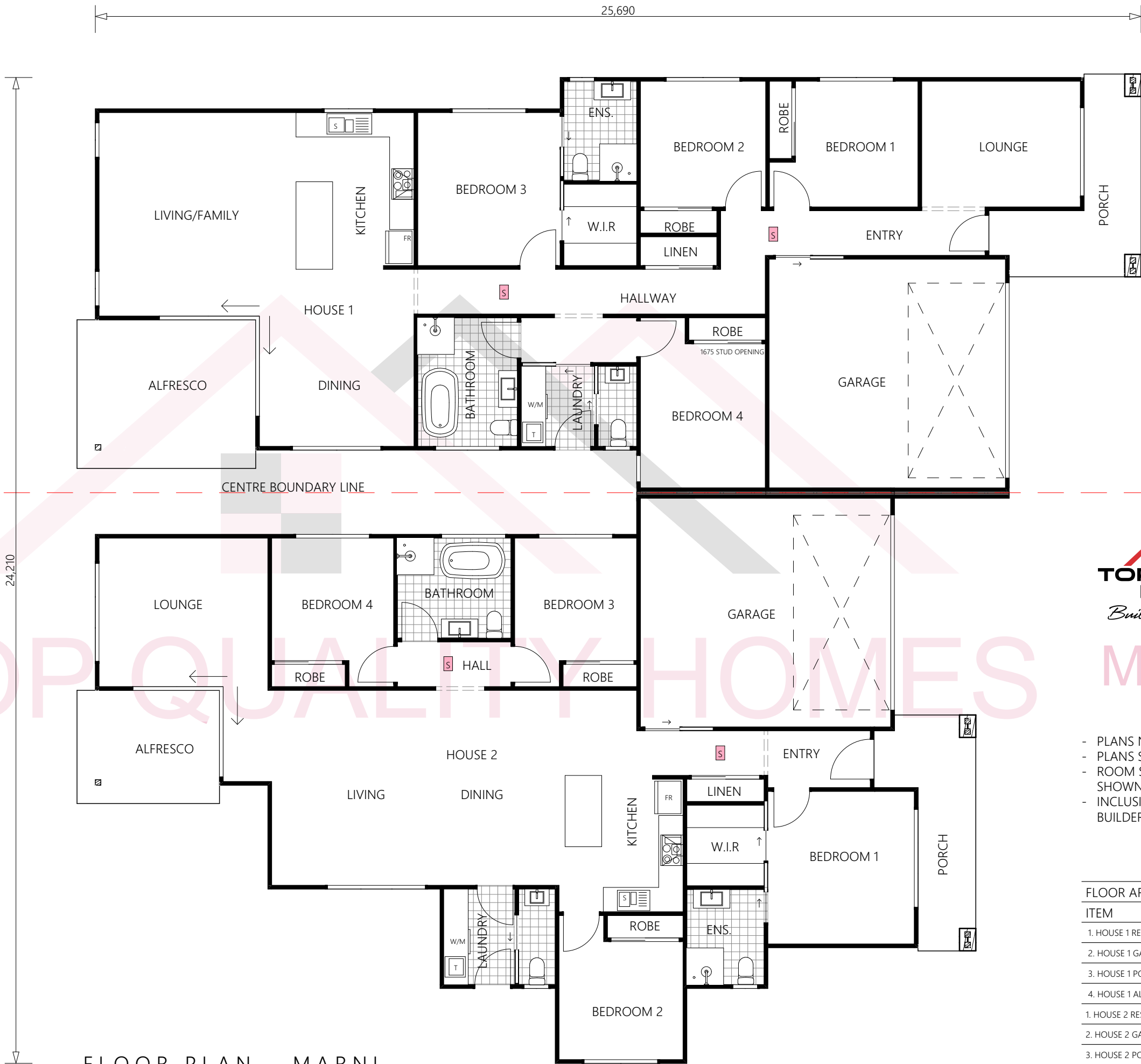
FLOOR PLAN - MARNI
